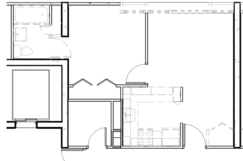
1 Unit Type 1 Demolition Plan 1/8" = 1'-0"
