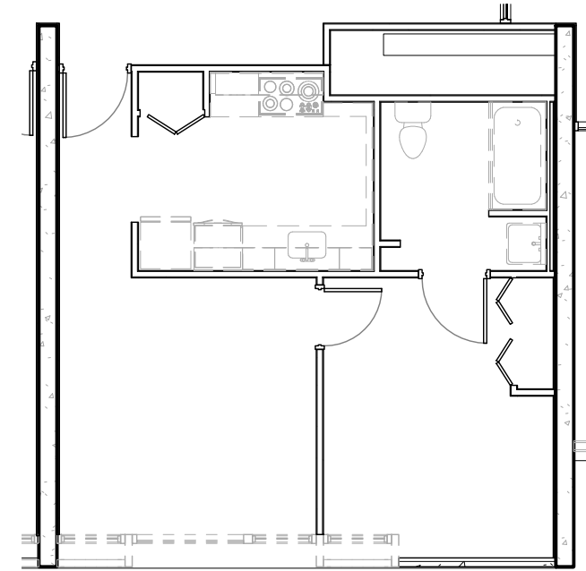
1 Unit Type 7A Demolition Plan 1/8" = 1'-0"
