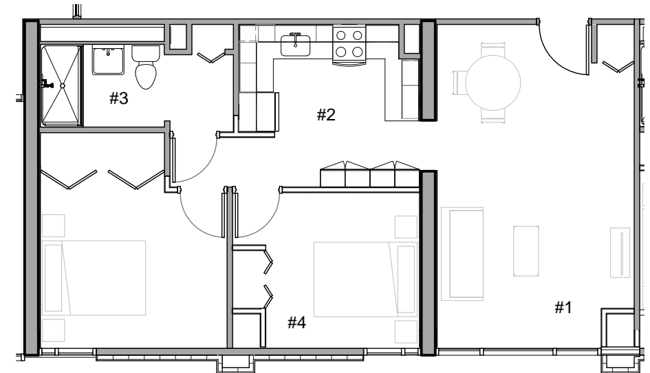
2 Unit Type 5A Proposed Plan 1/8" = 1'-0"
