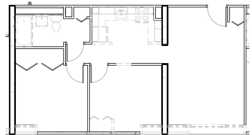
1 Unit Type 5 Demolition Plan 1/8" = 1'-0"
