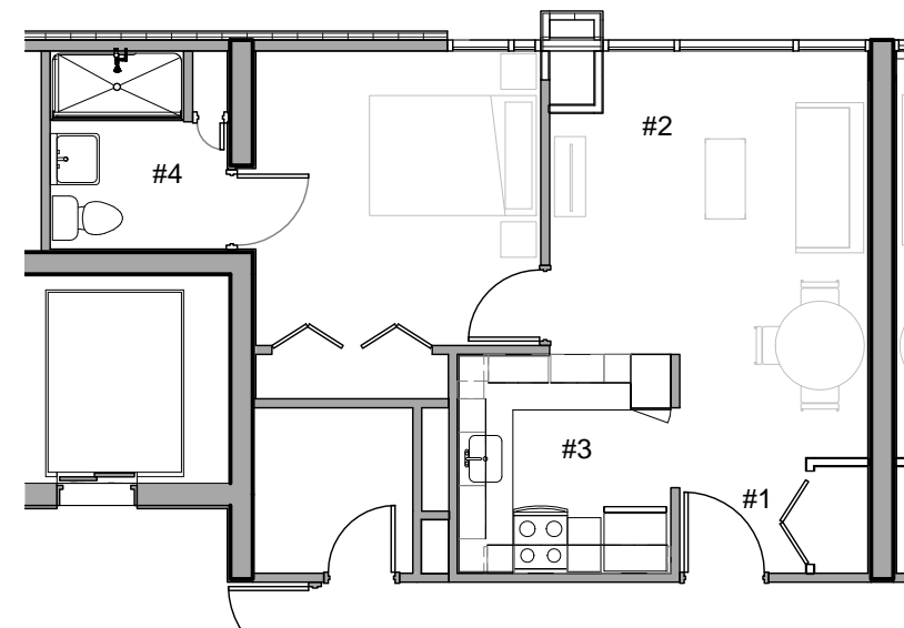
2 Unit Type 1 Proposed Plan 1/8" = 1'-0"
