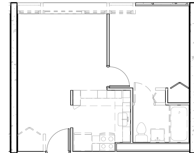
1 Unit Type 2 Demolition Plan 1/8" = 1'-0"
