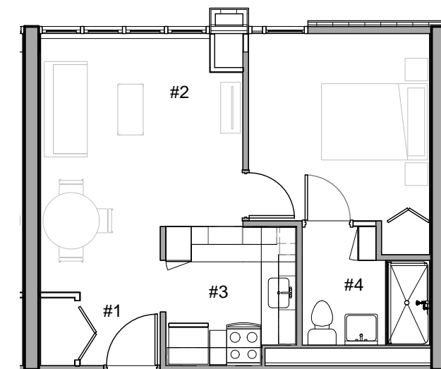
2 Unit Type 2 Proposed Plan 1/8" = 1'-0"
