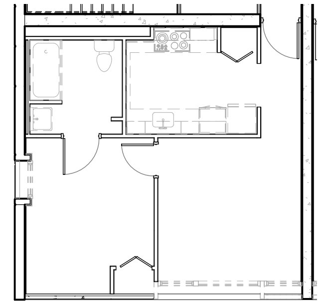
1 Unit Type 7B Demolition Plan 1/8" = 1'-0"
