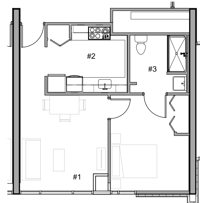
2 Unit Type 7A Proposed Plan 1/8" = 1'-0"
