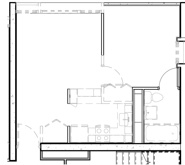
1 Unit Type 3 Demolition Plan 1/8" = 1'-0"
