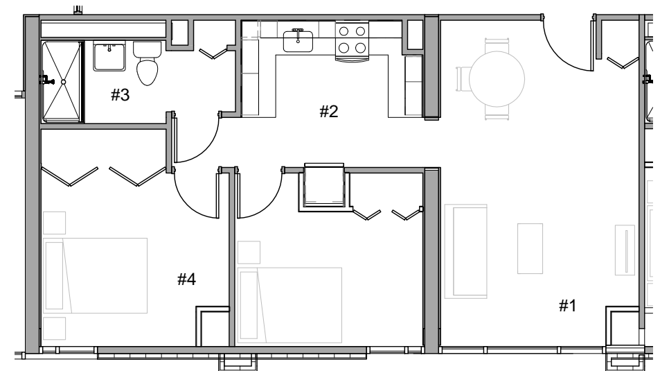
2 Unit Type 5 Proposed Plan 1/8" = 1'-0"
